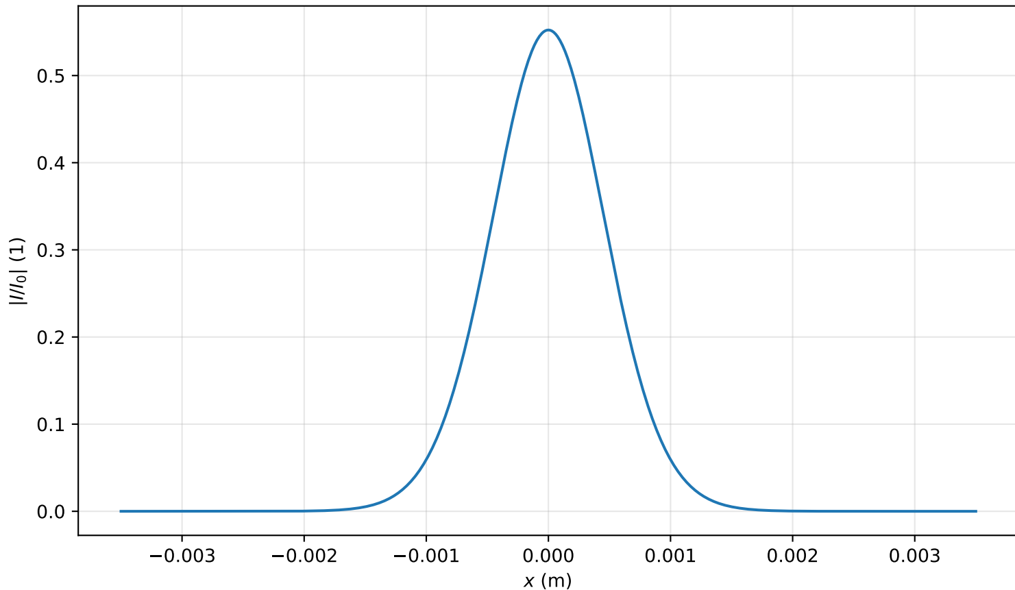
Intensity profile I(x, y = 0, z = 2.149m)/I_0 , P_{in}=0.2P_{cr} , artificial time
